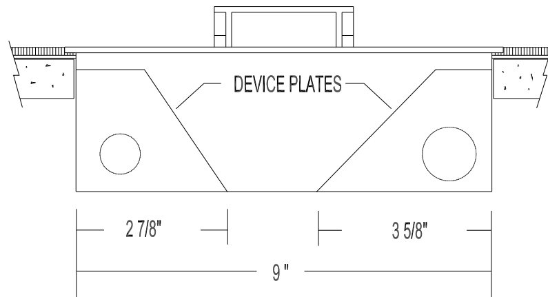
END VIEW
