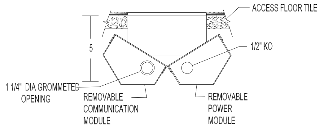
END SECTION
