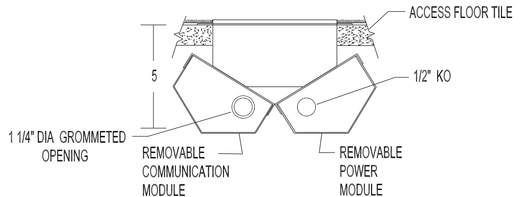
END SECTION
