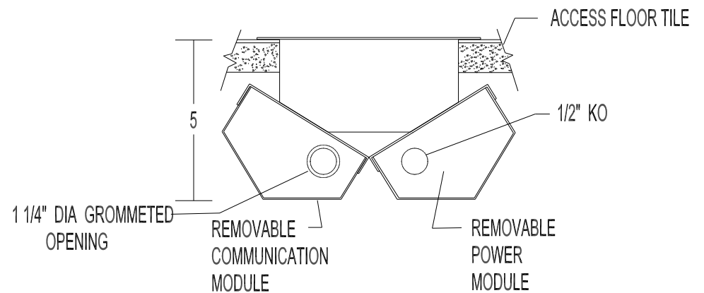
END SECTION
