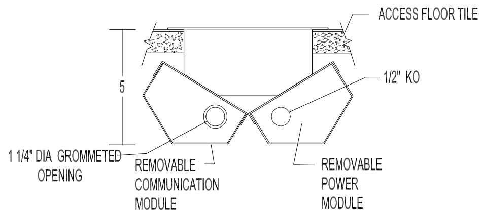
END SECTION
