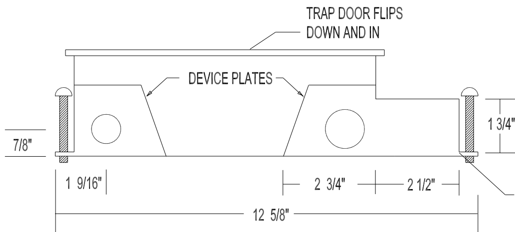
END VIEW
