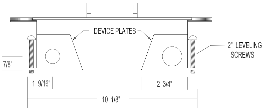
END VIEW
