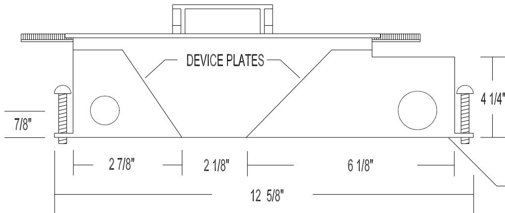
END VIEW
