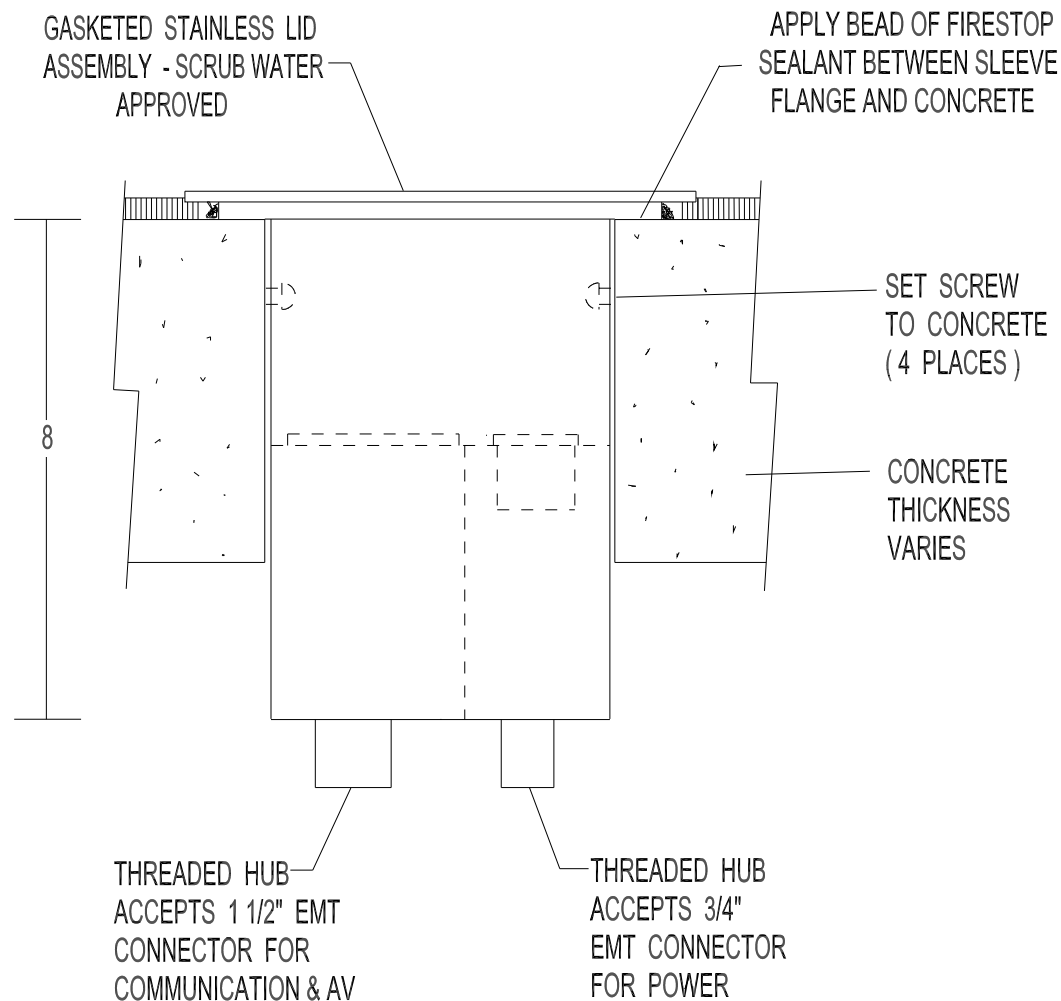
SIDE SECTION
